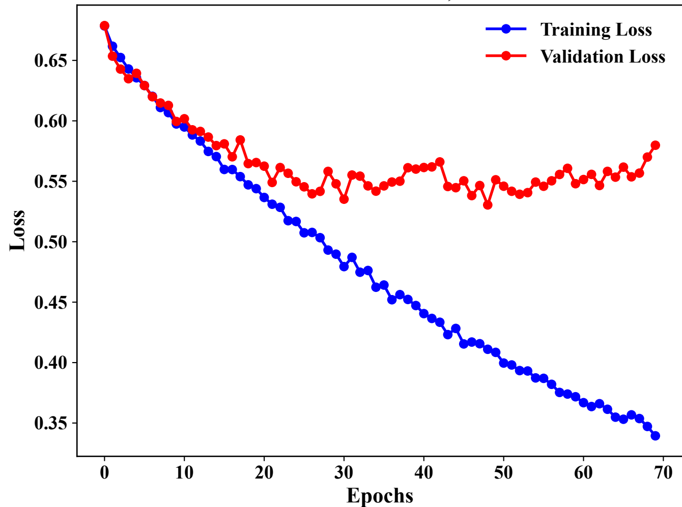
Loss Curves: Seed 24, Rank 1
